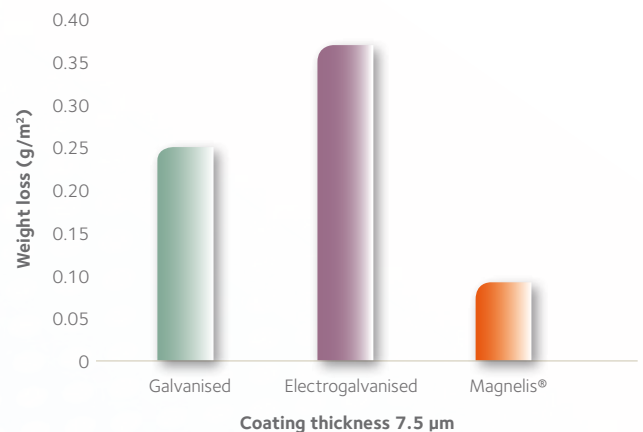
Lubrication: Fuchs 4107S in excess Powdering behaviour comparison between metallic coatings expressed in weight loss (g/m²)
